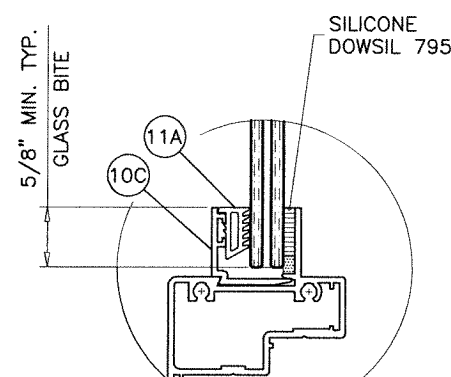
ALT. GLAZING OPTION
