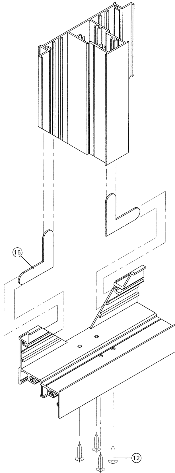
IMPOST CORNER
