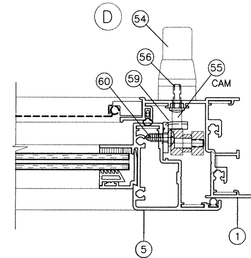
CAM LOCKS OPTION
